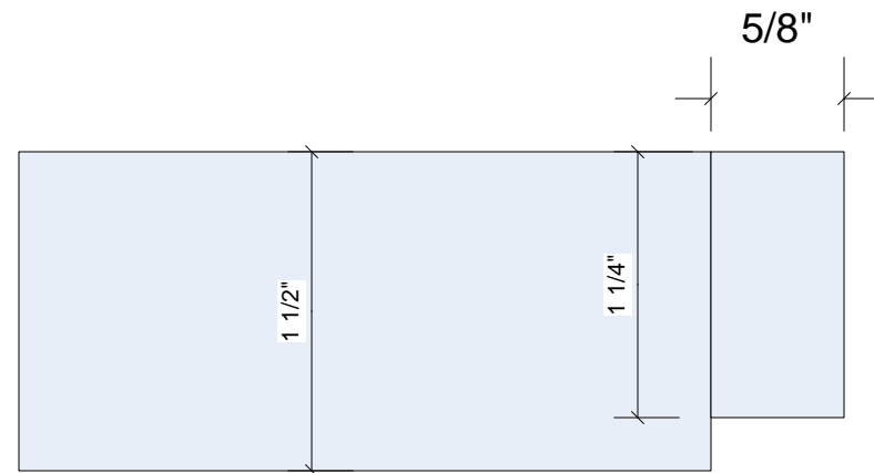
Stretcher Detail – Side View
